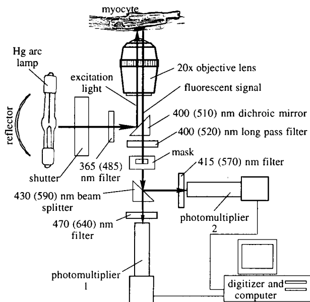
FIGURE 1 Schematic diagram of the microfluorimeter. Light from a 100-W mercury arc lamp was passed by a computer-operated shutter for 100 ms through condenser optics and a 10-nm-wide bandpass filter peaking at 365 nm to a dichroic mirror. The dichroic coating on the mirror reflects wavelengths shorter than 400 nm up through a 20\times Nikon fluorite objective lens (numerical aperture, 0.75) to illuminate the cells. The light from the total intrinsic cellular fluorescence is collected by the objective lens and passes through the 400-nm dichroic mirror and a 400-nm-long pass filter (blocks wavelengths shorter than 400 nm). A rotatable stage in conjunction with a maneuverable mask in the optical path blocks fluorescent light from all cells in the objective lens field except one. Fluorescent light from that cell passes to a second dichroic mirror, which serves as a beam splitter. The dichroic coating reflects light shorter than 430 nm to photomultiplier 2. Light longer than 430 nm passes to photomultiplier 1. Narrow bandpass filters pass light at 470 and 415 nm to photomultipliers 1 and 2, respectively. Filter and mirror wavelengths were changed to those shown parenthetically to determine intracellular pH with the dye SNARF-1.
