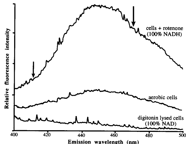
FIGURE 2 Fluorescent emission spectra of isolated heart cells. Fluorescence intensity as a function of emission wavelength was measured in stirred suspensions of heart cells in a Perkin-Elmer 650-40 fluorimeter. The excitation wavelength was 365 nm. After taking a spectrum of aerobic heart cells, 10 \mu\text{M} rotenone was added to give the maximum NADH signal. A separate portion of cells was lysed with digitonin. The signal from digitonin-lysed cells gives an emission spectrum identical to that observed with CCCP-treated cells corresponding to the minimum NADH signal. Arrows indicate the measuring wavelengths of the microfluorimeter.
