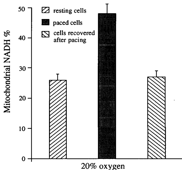
FIGURE 7 Effect of electrical stimulation on NAD reduction of hypoxic single heart cells. Cells ( 10 \times 10^4 /cm 2 ) were superfused with medium equilibrated with 20% \text{O}_2 /5% \text{CO}_2 . NAD reduction of resting cells was 26 \pm 2\% ( n = 30 cells; uV). Electrical stimulation significantly increased NAD reduction to 48 \pm 3\% ( n = 30 cells; uX); this effect differs markedly from that seen in well-oxygenated cells at lower cell density: 2 \times 10^4 /cm 2 and 95% \text{O}_2 /5% \text{CO}_2 (see Fig. 9). NAD reduction recovered to 27 \pm 2\% , nearly the original value, after 20 min of rest (uT).
