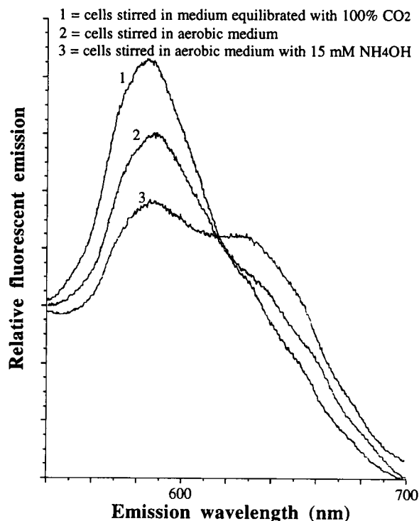
FIGURE 4 Fluorescent emission spectra from suspensions of SNARF-loaded myocytes. Cells were illuminated at 485 nm. Spectra were recorded with a Perkin-Elmer model 650-40 fluorimeter from stirred suspensions ( 1.25 \times 10^5 cells/ml) of SNARF-loaded heart cells (see Materials and Methods). Trace 2 shows the spectrum recorded from aerobic cells at pH_i 7.06 (see text). Upon acidification with media equilibrated with 100% CO_2 (trace 1), there was an increase in fluorescent emission at 585 nm, with an isoemissive point near 620 nm. When pH_i was increased with NH_4OH (trace 3), fluorescent emission at 585 nm was markedly decreased and fluorescent emission at 640 nm was increased.
