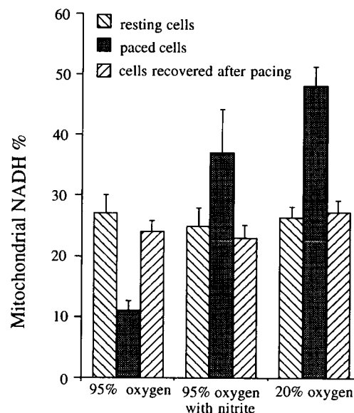
FIGURE 9 Summary of the effects of limited oxygen availability on NAD reduction of electrically stimulated single heart cells. Note that NAD reduction in electrically paced cells in oxygenated medium has decreased to 11%, but when oxygen supply is limited NAD reduction increases above control levels.
