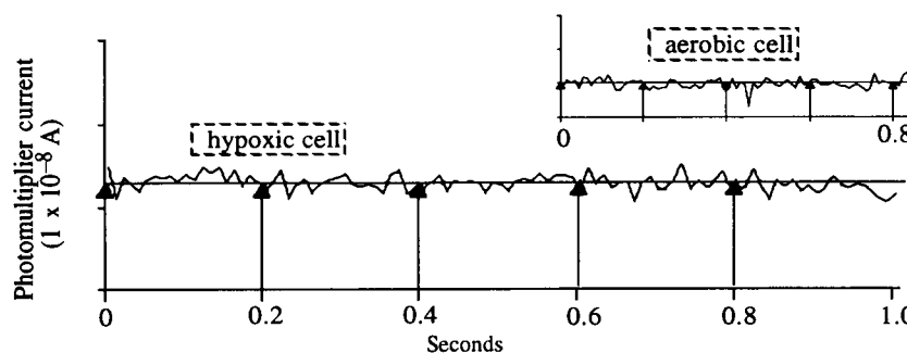
FIGURE 5 NADH fluorescence is not synchronized with cell contractions. The traces show the difference signal between 470 and 415 nm. Each cell was electrically stimulated to contract for at least 10 min with Pt-Ir field electrodes at the times indicated by the arrow. The inset shows a record from a cell superfused with medium equilibrated with 95% O 2 and 5% CO 2 ( aerobic cell ), stimulated at 5 Hz. The large trace shows a record from a cell superfused with medium equilibrated with 20% O 2 , 5% CO 2 , and 75% N 2 ( hypoxic cell ). During stimulation, the extent of NAD reduction in the hypoxic cell was greater than that in the aerobic cell. There is no detectable consistent change in mitochondrial NADH fluorescence correlated with the stimulation of either aerobic or hypoxic cells. We conclude that changes in NADH during cell contractions are not detectable on this time scale.
