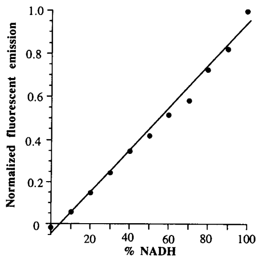
FIGURE 3 Fluorescence intensity is a linear function of the fraction of NADH. Fluorescence intensity (470–415 nm) normalized to the value recorded at 100% NADH ( ordinate ) was recorded from solutions of NADH plus NAD in hollow glass slides, the dimensions of which were similar to those of a heart cell. The fitted line is a linear regression to the data.
