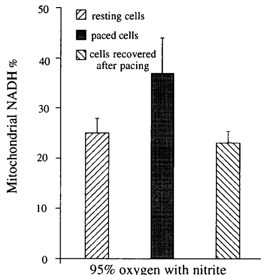
FIGURE 8 Effect of myoglobin inactivation on NAD reduction of electrically stimulated single heart cells. Cells ( 2 \times 10^4 /cm 2 ) were superfused with medium containing 2 mM sodium nitrite and equilibrated with 95% O_2 /5% CO_2 . NAD reduction of resting cells was 25 \pm 3\% ( n = 48 cells; uV). Electrical stimulation significantly increased NAD reduction to 37 \pm 7\% ( n = 48 cells; uX), an effect markedly different from that seen in well-oxygenated cells at the same cell density. NAD reduction recovered to 23 \pm 2\% , nearly the original value, after 20 min of rest (uT).
